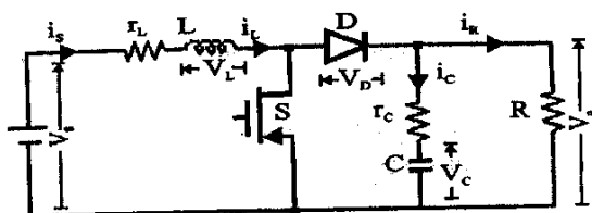
Fig.1 : Boost converter power circuit elements
